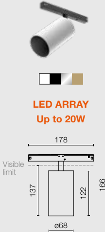
LIGHT SHADOW SPOT 60
