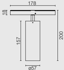
LED ARRAY 22,5W
